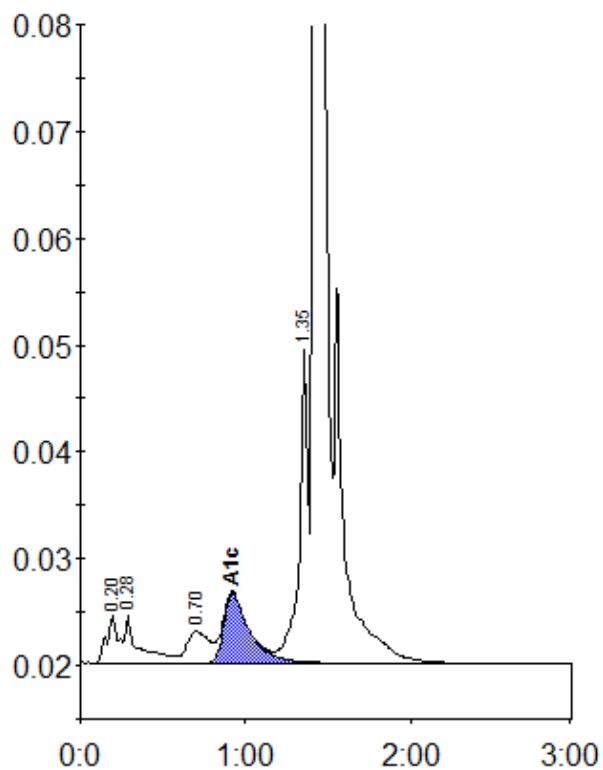
Peak table - ID: 10554459
